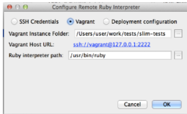
Creating vagrant-based remote sdk
